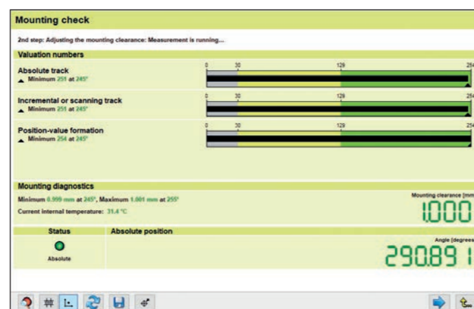
Mounting accuracy with the PWM 21 and the ATS software
