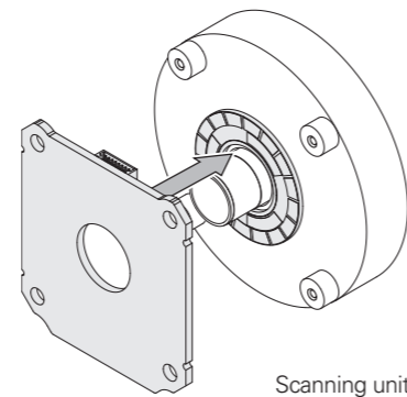
Scanning unit
